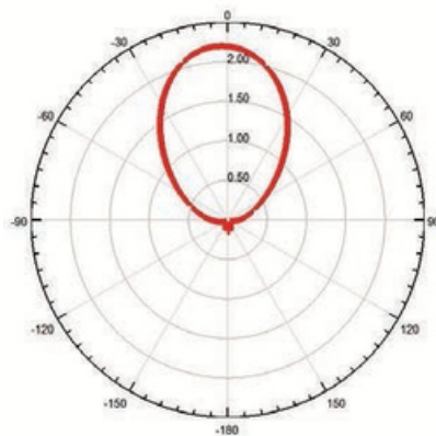
Radiation Pattern 2
