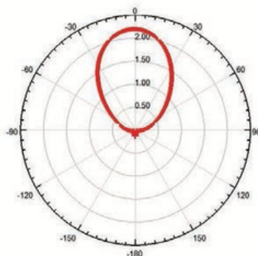
Radiation Pattern 1
